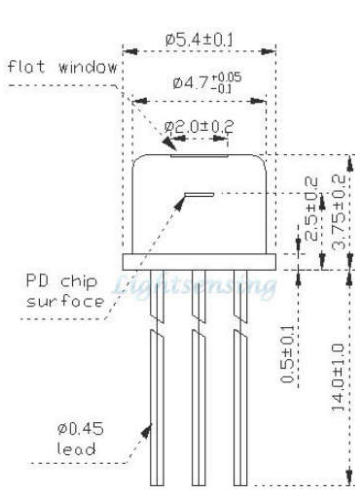
2mm flat window TO Model: 0
