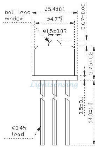
Standard ball lens cap TO Model: 1
