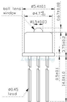
Standard ball lens TO
