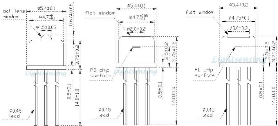
Standad ball lens TO Model: 1
